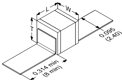
Micro-strip ribbon leads (Type 1)
