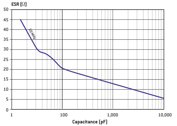
4040: TYPICAL ESR VERSUS CAPACITANCE
