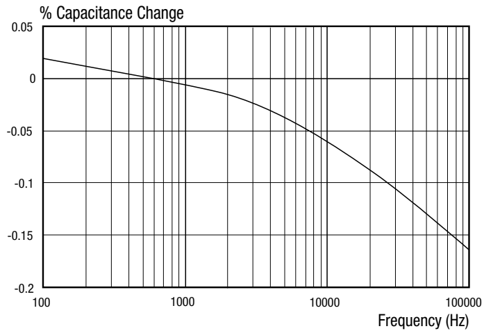
CAPACITANCE CHANGE VS. FREQUENCY - METALIZED POLYPROPYLENE
