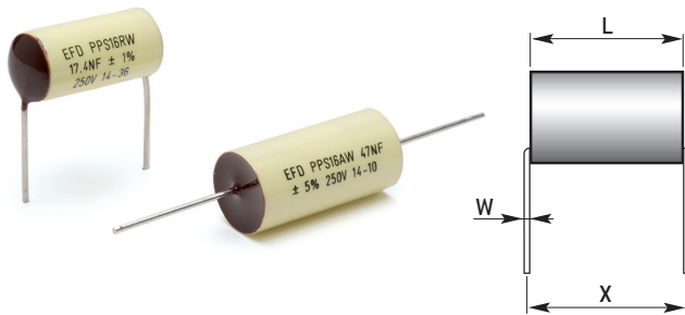
Radial leads Model PP 16 R
