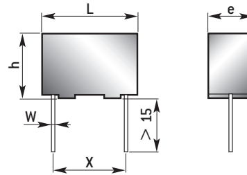
Radial leads Models PS • 3 - PS • 4
